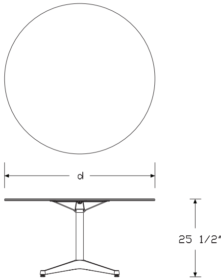
Contract Base
