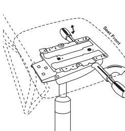
Advanced synchro tilt w/ side tension knob - ASA7
