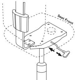
Controls Swivel tilt - SWT2
