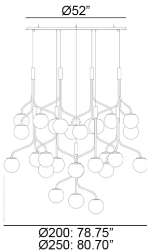
Pictured: Curve Cluster Group of 5 Small Pendants - Glass Shades Ø200
