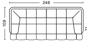
QLT2A | 2.5 SEATER WIDTH 248 CM | 97.5" DEPTH 109 CM | 42.9" HEIGHT 72 CM | 28.5" SEAT HEIGHT 41 CM | 16.25" SEAT DEPTH 77 CM | 30.25"
