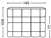
QLT6FS | FREESTANDING WIDE WIDTH 145 CM | 54.7" DEPTH 109 CM | 42.9" HEIGHT 72 CM | 28.5" SEAT HEIGHT 41 CM | 16.25" SEAT DEPTH 77 CM | 30.25"
