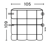
QLT4 | NARROW MIDDLE MODULE WIDTH 105 CM DEPTH 109 CM HEIGHT 72 CM SEAT HEIGHT 41 CM SEAT DEPTH 77 CM
