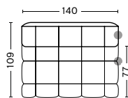
QLT10L | WIDE END MODULE | LEFT W/O ARMREST WIDTH 140 CM DEPTH 109 CM HEIGHT 72 CM SEAT HEIGHT 41 CM SEAT DEPTH 77 CM
