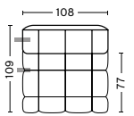
QLT8R | NARROW MODULE | RIGHT W/O ARMREST WIDTH 108 CM DEPTH 109 CM HEIGHT 72 CM SEAT HEIGHT 41 CM SEAT DEPTH 77 CM
