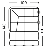
QLT5L | CHAISE LONGUE MODULE | LEFT WIDTH 109 CM DEPTH 143 CM HEIGHT 72 CM SEAT HEIGHT 41 CM SEAT DEPTH 111 CM
