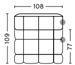
QLT8L | NARROW END MODULE | LEFT W/O ARMREST WIDTH 108 CM DEPTH 109 CM HEIGHT 72 CM SEAT HEIGHT 41 CM SEAT DEPTH 77 CM
