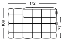
QLT7R | CHAISE LONGUE MODULE | RIGHT WIDTH 172 CM DEPTH 109 CM HEIGHT 72 CM SEAT HEIGHT 41 CM SEAT DEPTH 77 CM
