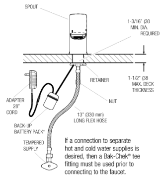
EFX-300.00X.0X1X Faucet with Single Line Water Supply
