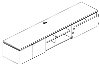
Float Edge Top, 1-1/2" Thick Hinged Doors/ Shelves/ Flip Door 90" & 96"W, 20D (left hand shown)
