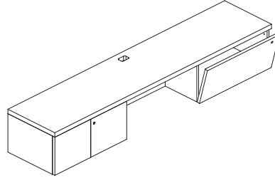
Square Edge Top, 1-1/2" Thick Hinged Doors/ Open/ Flip Door 90" & 96"W, 20D (left hand shown)
