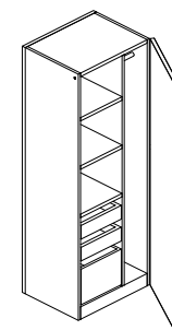
Shelves, BBF Drawers, & Wardrobe Widths: 24" Depths: 20", 24"
