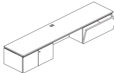
Float Edge Top, 1-1/2" Thick Hinged Doors/ Open/ Flip Door 90" & 96"W, 20D (left hand shown)
