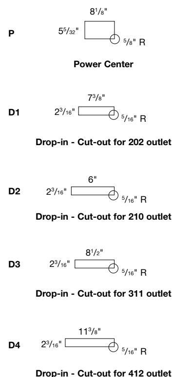
Figure 2: Cut-out Sizes
