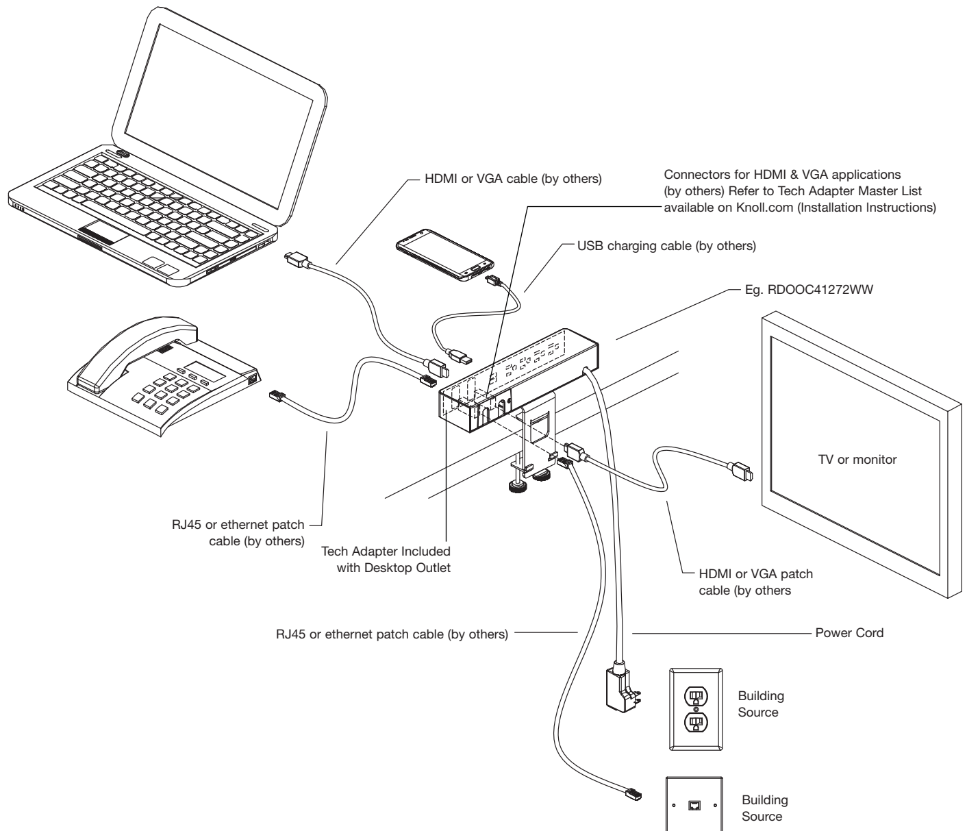
Figure 17 Cabling Diagram
