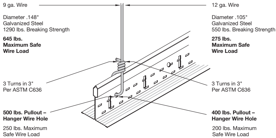
9-gauge Wire-Breaking Strength and Technical Data
