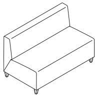
Overall: 28"D 50"W 29½"H Inside: 20"D 50"W 12¼"H Seat: 17¼"H Angle Degree: 0°
