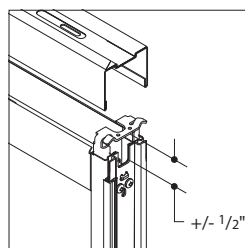
Mortise Cylindrical
