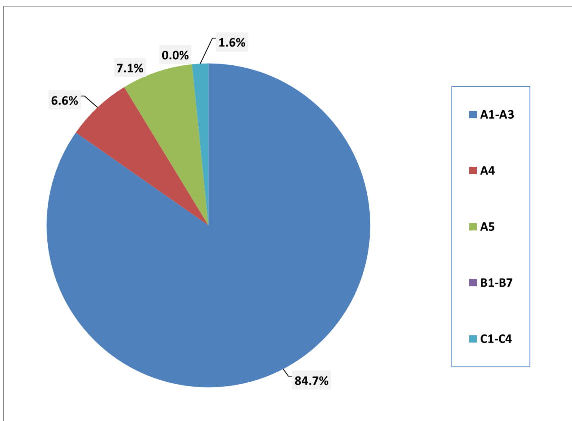
Figure 3: Process Dominance Analysis for GWP for the Production of 1 Square Foot of 7/8 in. Mars™ High-NRC (85/35/90) Acoustical Ceiling Panels
