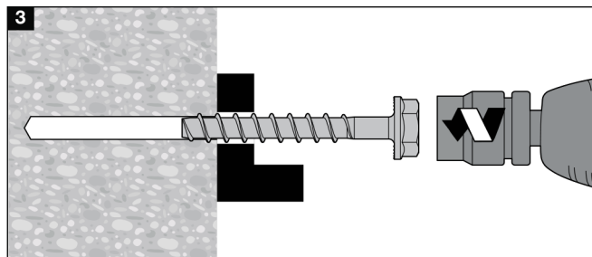
Fasten anchor tightly against fastened part.
