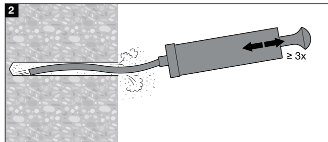
Clean drilled hole to remove debris.
