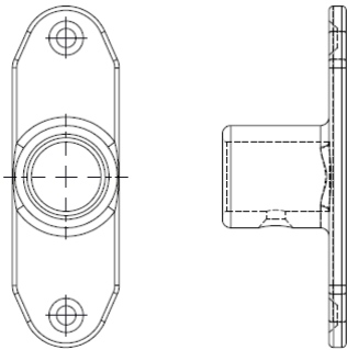
Part # OPTS-P03 Ceiling Vertical Mount Plate
