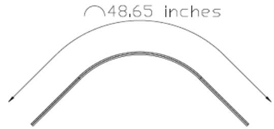
Part# OPTS- K1R03 90° Reversed 1 Ft Radius Track
