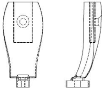
Part # OPTS-E03 Hanger & Track Connector
