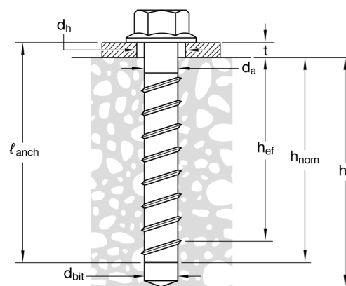
Figure 1 — KWIK HUS-EZ anchor installation details
