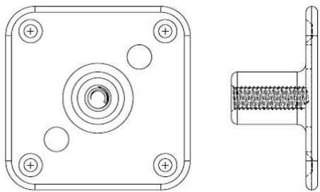
Part # OPTS-B03 Hard Ceiling Mounting Plate
