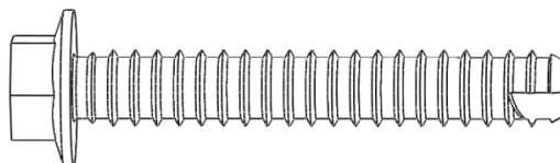
Part# OPTS-AN-C 1/4" x 2 5/8" Anchor for Concrete and Masonry
