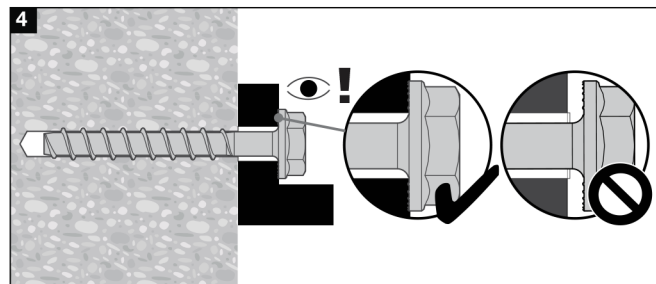
Install anchor using proper impact tool or torque wrench.
