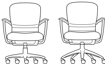
Standard Steel Base High Arc Base Standard or High Arc Base seat height (15"-20" (381mm-508mm))
