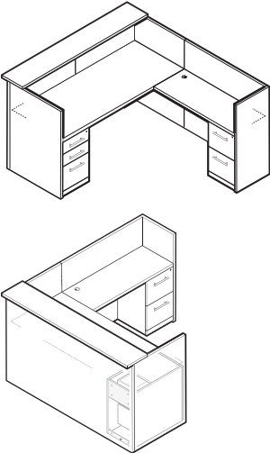
XZLR-RB (Right-hand shown)
