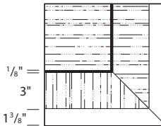
2.75"(70mm) edge and Border with Inlay Option (O) and mitered corner construction.
