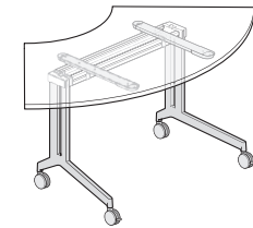
Crescent: Flip Table Top
