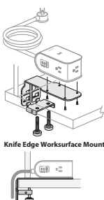
EUCB-TJP Knife Edge Worksurface Mount
