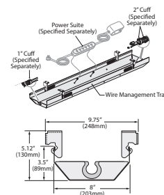
EUWT Wire Management Tray
