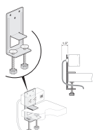
EUFB-0000-SB Classic Power Module Bracket - Vertical Bracket
