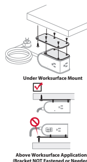
EUUB-UP Above Worksurface Application
