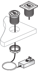
EURT-0072-1010 EURT-00E4-1010 Bezel Utility Model USB Charging: Round or Square
