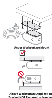
EUUB-UP Above Worksurface Application
