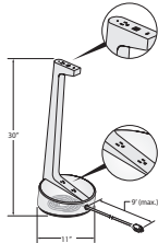
EUCN-PJ Collaborative Power Station
