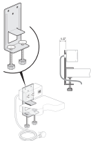
EUFB-0000-SB Classic Power Module Bracket - Vertical Bracket
