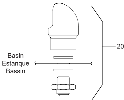
VANDAL RESISTANT BUBBLER DETAIL
