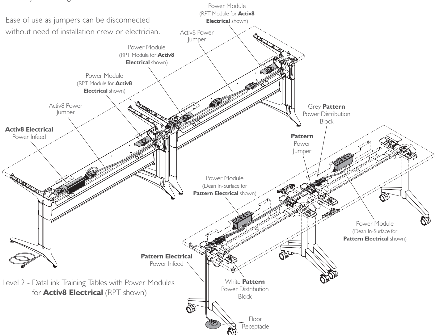
Level 2 - Pirouette Tables with Power Modules for Pattern Electrical (Dean In-Surface shown)
