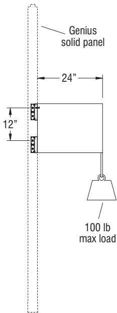
24" Deep Cabinet/Casegoods (side view)
