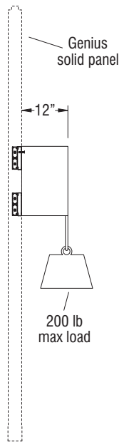
12" Deep Cabinet/Casegoods (side view)
