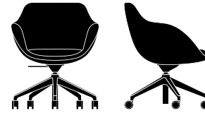
68736 Side chair with arms and 5-star aluminum base W 27" D 25.5" H 32.25"– 36.75" SH 17.75"– 22.25" AH 9"
