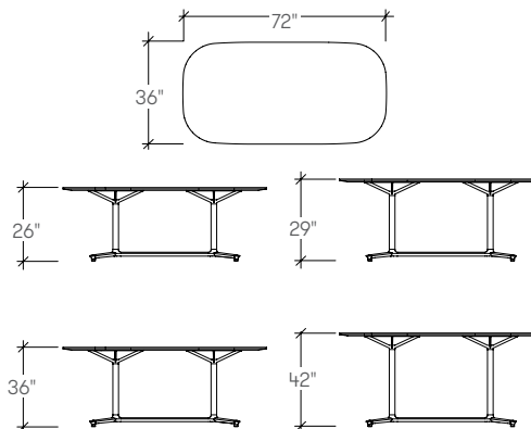
Bevy Rectangular Work Y Pedestal Table (STETK)
