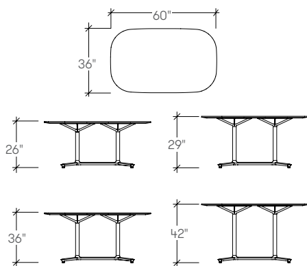
Bevy Rectangular Work Y Pedestal Table (STETK)
