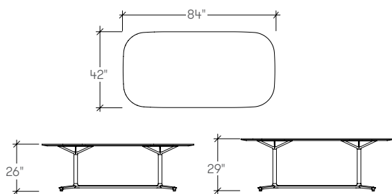
Bevy Rectangular Work Y Pedestal Table (STETK)
