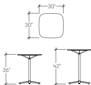
Bevy Square Cafe Pedestal Table (STETH)
