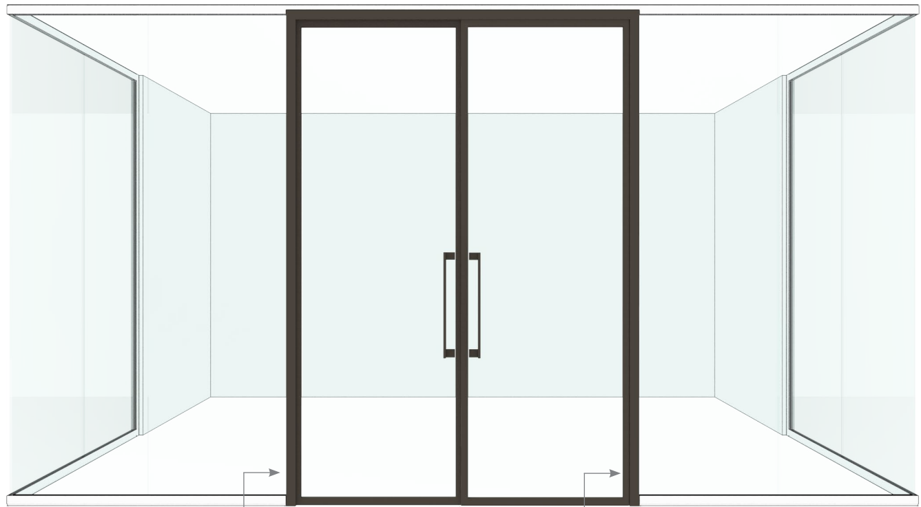
Pivot Door Jamb Connection (FVDJPC)
