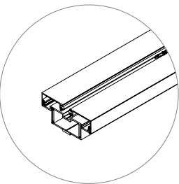
F W B F S O Base Frame Assembly, Single Offset
