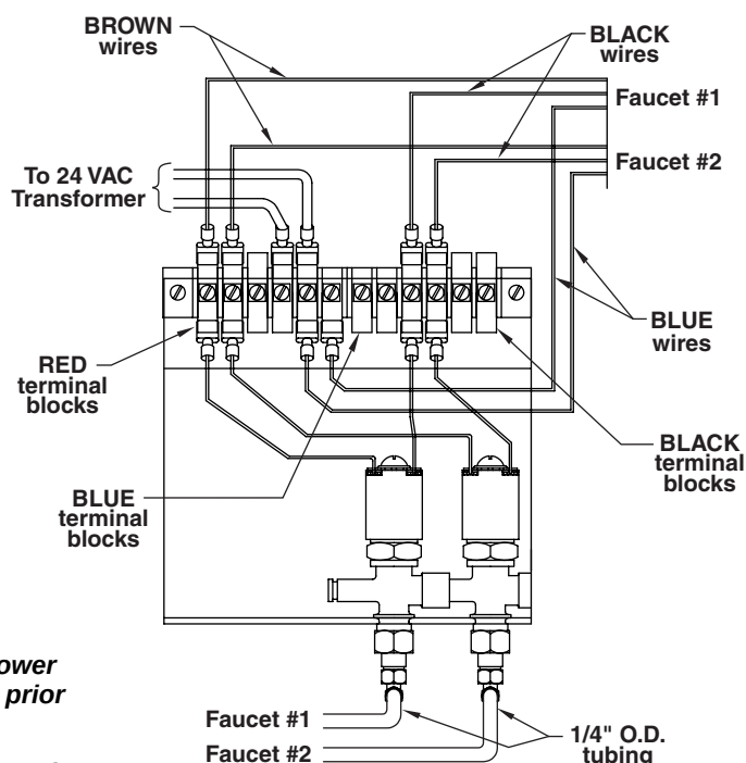
Dual-Faucet Installation
