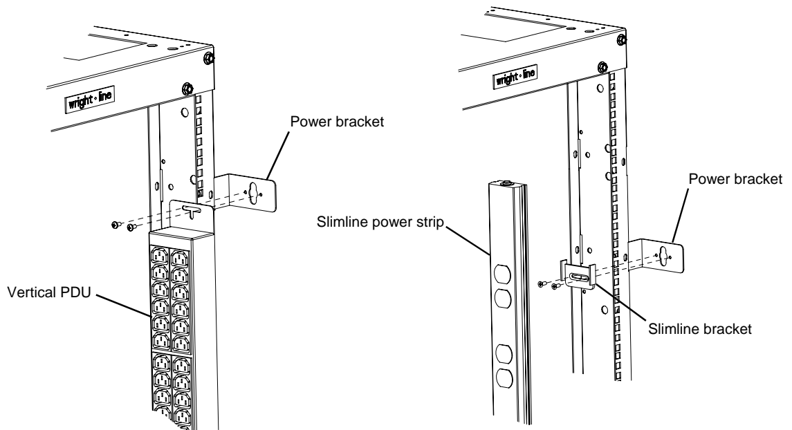
Figure 3 Mounting Vertical PDU
