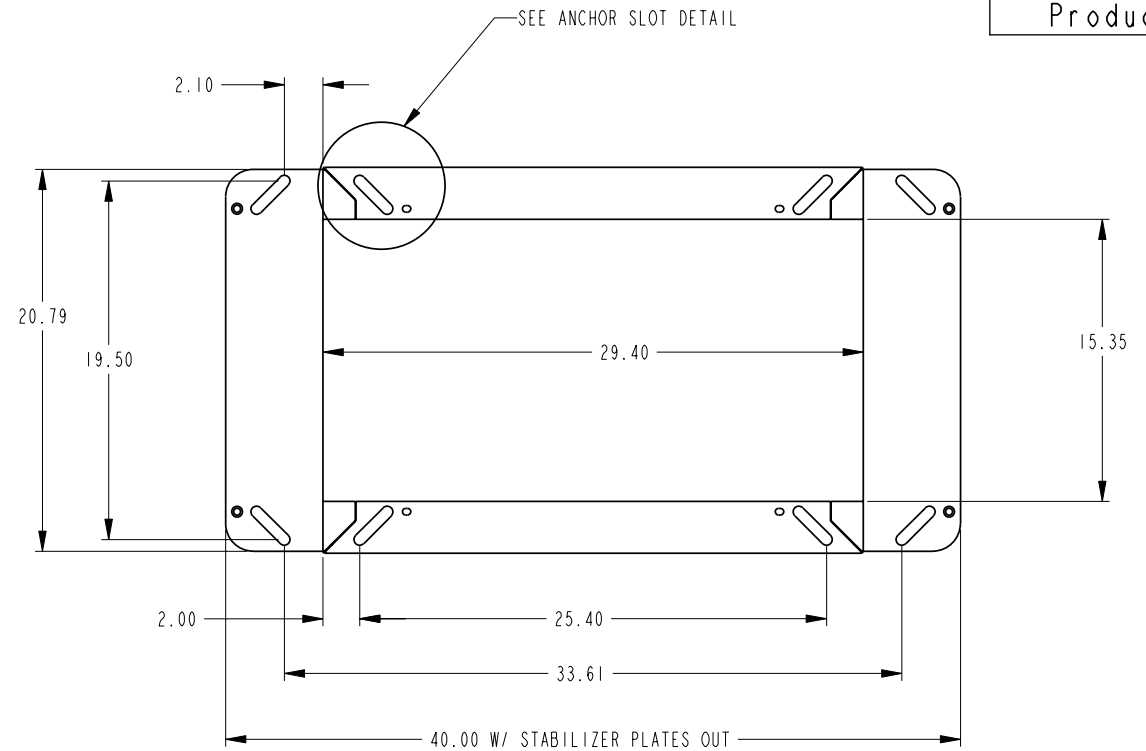
BOTTOM VIEW
