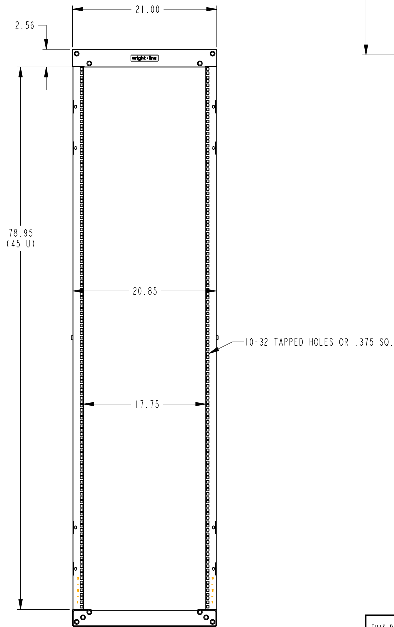
FRONT VIEW
