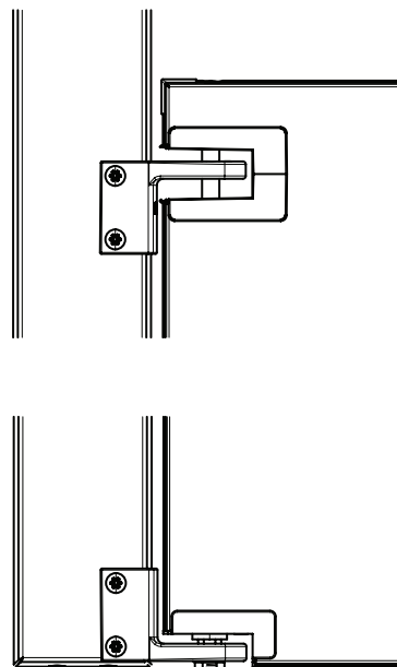
Finished View of Bottom Hinge
