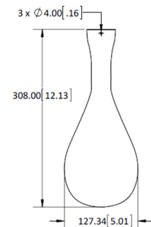
DIMENSIONS ARE IN MILLIMETERS [INCHES] (NOT TO SCALE)
