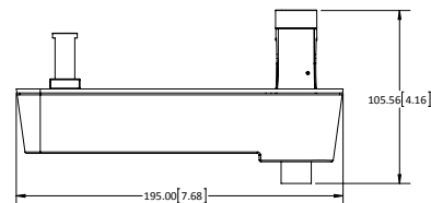
(29) HOUSING ADAPTER FOR P-TRACK
