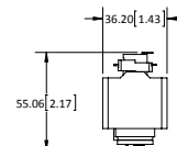
(28) J-TRACK ADAPTER
