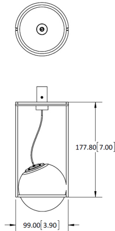
DIMENSIONS ARE IN MILLIMETERS [INCHES] (NOT TO SCALE)
