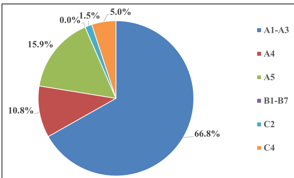
Figure 4: Process Dominance Analysis for the Production of 1 MSF of 1/4 in. (6.4 mm) Sheetrock® Brand Flexible Gypsum Panels
