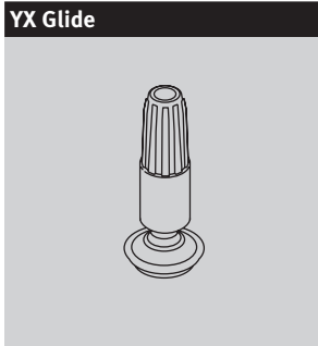
YX Glide 1 7/8-inch-high glide; black nylon stem; steel-plated swivel foot with Floor Saver Glide™ insert; for use on hard floors only Applicable on: Caper Chairs
