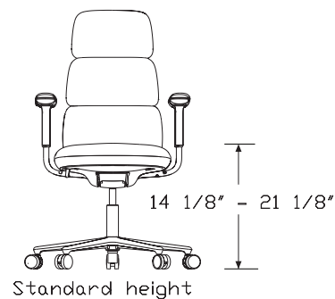
Standard height
