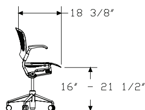
FLEXNET Seat
