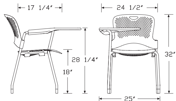
Flexnet Seat
