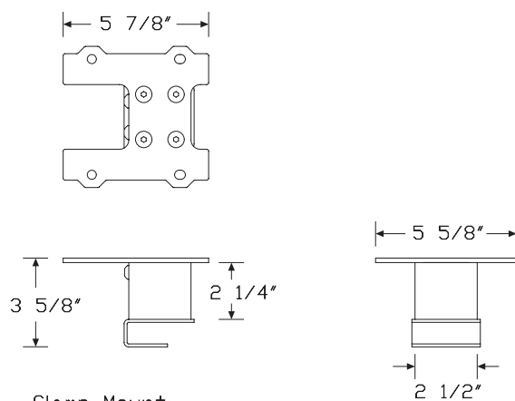
Clamp Mount
