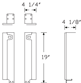
Wooden Attachments
