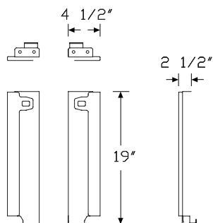
Metal Attachments
