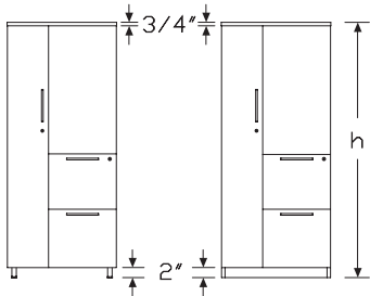
Foot Base File/File, Wardrobe Left
