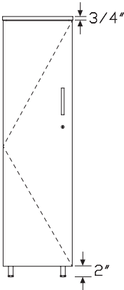
Left-Hinged Door Front with Tube Foot
