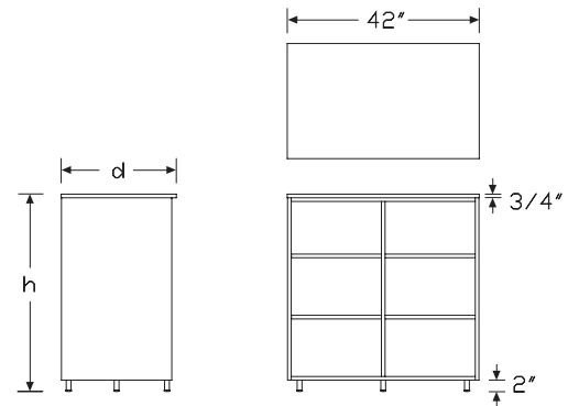
With Center Divider
