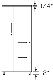
Tube Foot File/File, Wardrobe Left
