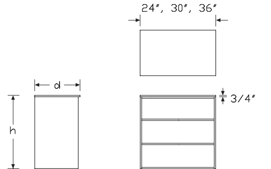
Without Center Divider
