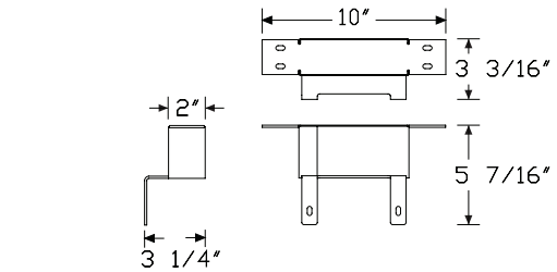
attached stanchion
