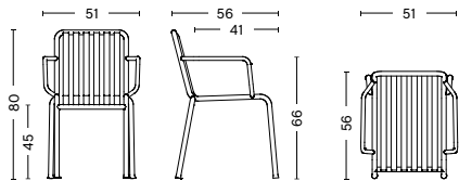
PALISSADE ARMCHAIR Width 51 cm Depth 56 cm Height 80 cm Seat height 45 cm Seat depth 41 cm Weight 20lbs
