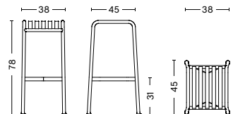
PALISSADE BAR STOOL Width 38 cm Depth 45 cm Height 78 cm Weight 18lbs
