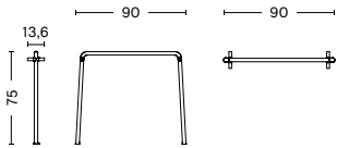
PALISSADE MIDDLE LEG Width 90 cm Depth 13,5 cm Height 75 cm Weight 8lbs
