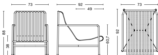
PALISSADE LOUNGE CHAIR HIGH Width 73 cm Depth 92 cm Height 88 cm Seat height 38 cm Seat depth 49 cm Weight 40lbs
