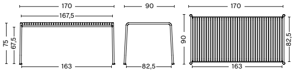
PALISSADE TABLE Length 170 cm Width 90 cm Height 75 cm Weight 70lbs
