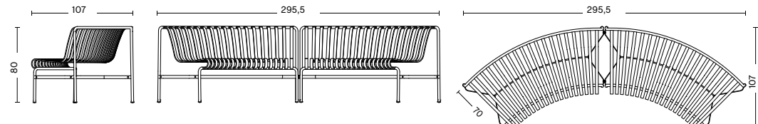
PALISSADE PARK DINING BENCH | IN/IN | SET OF 2 Width 295,5 cm Depth 107 cm Height 80 cm Seat height 45 cm Seat depth 44 cm Weight 102lbs
