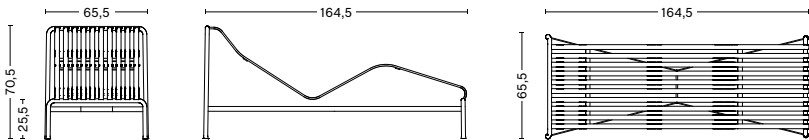
PALISSADE CHAISE LOUNGE Width 65,5 cm Depth 164,5 cm Height 70,5 cm Seat height 25,5 cm Weight 50lbs
