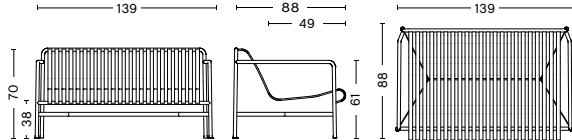
PALISSADE LOUNGE SOFA Width 139 cm Depth 88 cm Height 70 cm Seat height 38 cm Seat depth 49 cm Weight 67lbs
