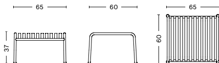
PALISSADE OTTOMAN Width 65 cm Depth 60 cm Height 37 cm Weight 20lbs
