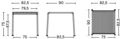
PALISSADE TABLE Length 82,5 cm Width 90 cm Height 75 cm Weight 39lbs
