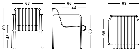
PALISSADE DINING ARMCHAIR Width 63 cm Depth 66 cm Height 80 cm Seat height 45 cm Seat depth 44 cm Weight 24lbs
