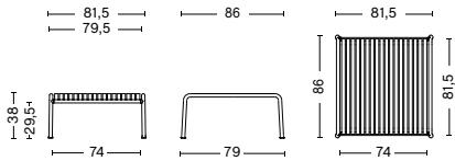
PALISSADE LOW TABLE Length 81,5 cm Width 86 cm Height 38 cm Weight 39lbs
