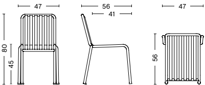
PALISSADE CHAIR Width 47 cm Depth 56 cm Height 80 cm Seat height 45 cm Seat depth 41 cm Weight 17lbs
