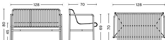
PALISSADE DINING BENCH Width 128 cm Depth 70 cm Height 80 cm Seat height 45 cm Weight 44lbs
