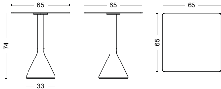
PALISSADE CONE TABLE, SQUARE Length 65 cm Width 65 cm Height 74 cm Base Diameter 33 cm Weight 84lbs
