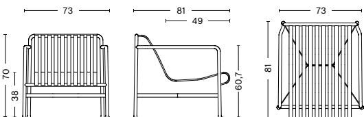
PALISSADE LOUNGE CHAIR LOW Width 73 cm Depth 81 cm Height 70 cm Seat height 38 cm Seat depth 49 cm Weight 35lbs
