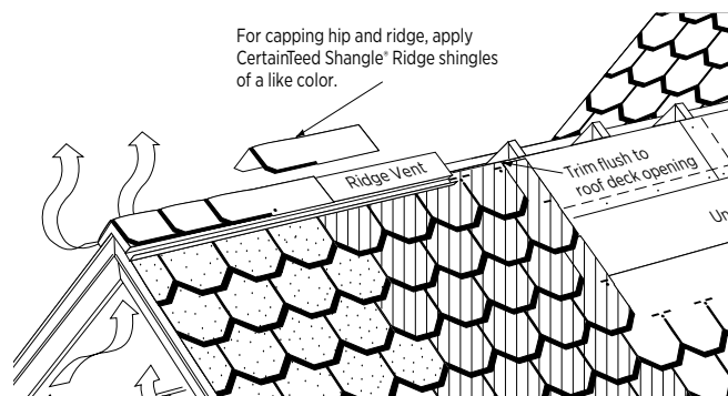
Figure 17-20: Installation of Shangle Ridge shingles on ridge vent.
