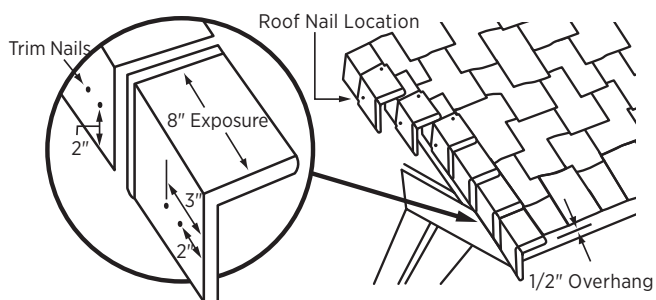
Figure 11-18: Rake edge application
