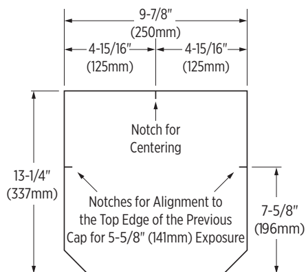
Metric Dimension
