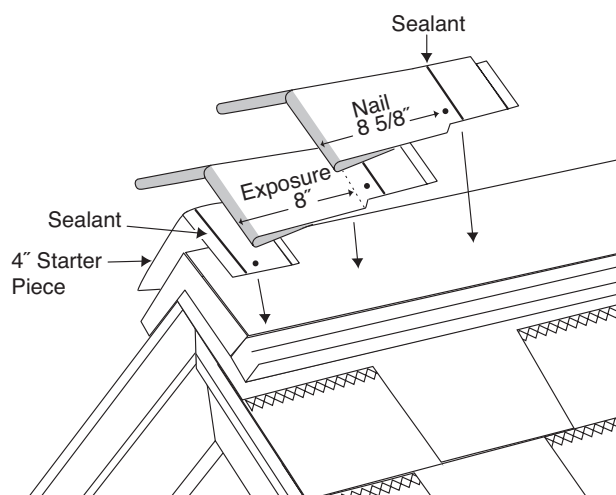
Figure 12-16: Hip and ridge application.
