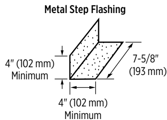
Figure 13-10: Step flashing minimum dimensions.
