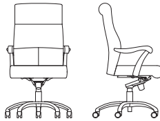
4875 High Back, Syncro-Tilt, Casters, Pneumatic Height Adjustment, Urethane Arm Cap, Wood Sleeve W 27.25" D 28" H 45.75–48.75" SH 19.25–22.25" AH 26.75–29.75"
