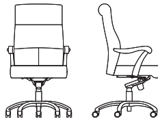
4872 High Back, Syncro-Tilt, Casters, Pneumatic Height Adjustment, Upholstered Arm Cap, Wood Sleeve W 27.25" D 28" H 45.5–48.5" SH 19.25–22.25" AH 27–30"
