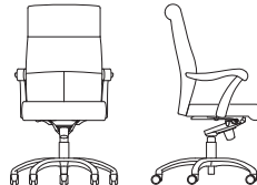
4772 High Back, Syncro-Tilt, Casters, Pneumatic Height Adjustment, Upholstered Arm Cap, Urethane Sleeve W 26.25" D 27.5" H 45.5–48.5" SH 19.25–22.25" AH 27–30"
