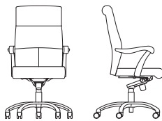
4775 High Back, Syncro-Tilt, Casters, Pneumatic Height Adjustment, Urethane Arm Cap, Urethane Sleeve W 26.25" D 27.5" H 45.5–48.5" SH 19.25–22.25" AH 26.75–29.75"
