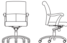
4762 Mid Back, Syncro-Tilt, Casters, Pneumatic Height Adjustment, Upholstered Arm Cap, Urethane Sleeve W 26.25" D 27.25" H 39.5–42.5" SH 19.25–22.25" AH 27–30"
