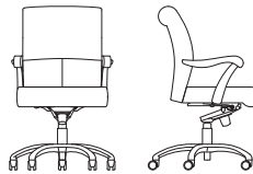
4862 Mid Back, Syncro-Tilt, Casters, Pneumatic Height Adjustment, Upholstered Arm Cap, Wood Sleeve W 27.25" D 27.5" H 39.5–42.5" SH 19.25–22.25" AH 27–30"
