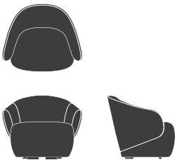
99020 Swish lounge chair with caster base Total height: 28.5" Seat height: 16" Total width: 34.75"
