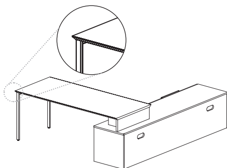
Peninsula desk with reverse bevel edge
