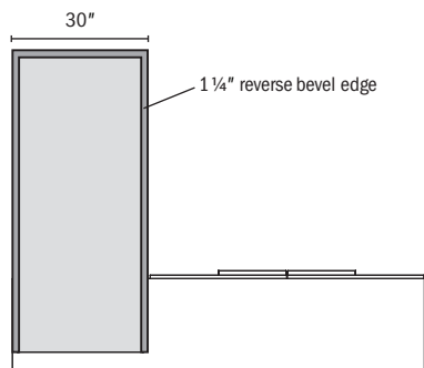
Plan view of peninsula with reverse bevel edge
