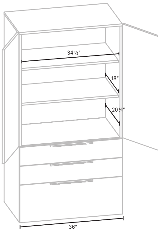
36"w upper storage compartment cabinet
