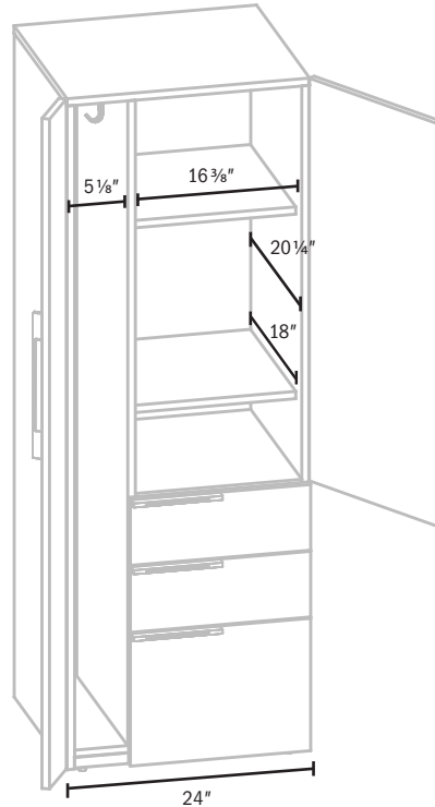
24"w side wardrobe with upper storage compartment
