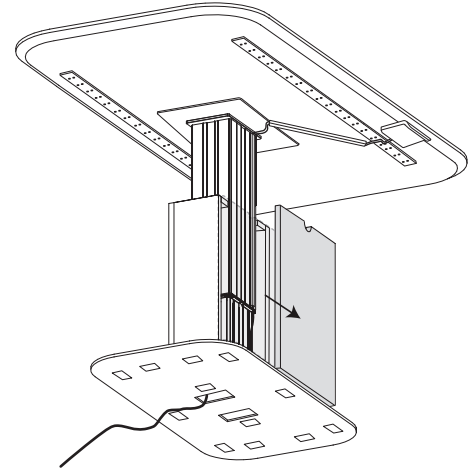
Electrical cord exits through the bottom side of the plate. Neoprene leveling pads allow the cord to lay flat.
