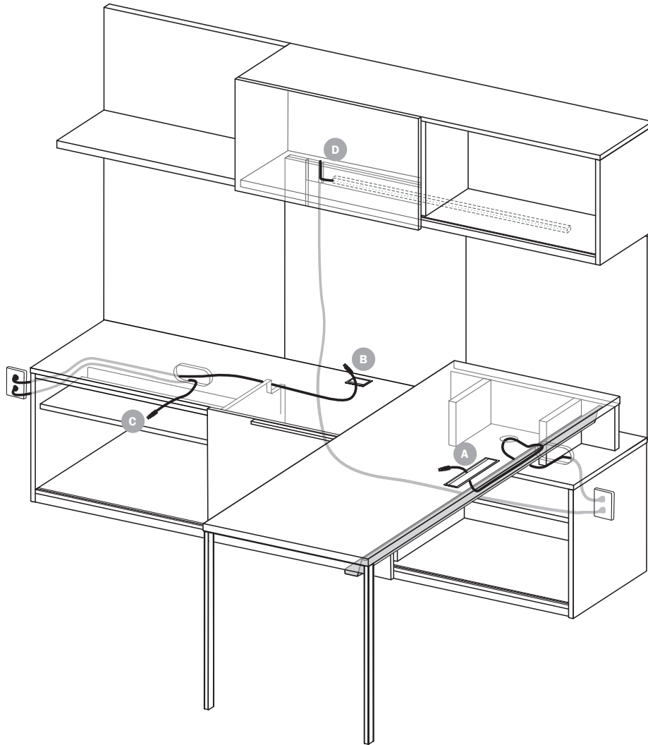
Adjustable Height Peninsula Desk with Secondary Storage
