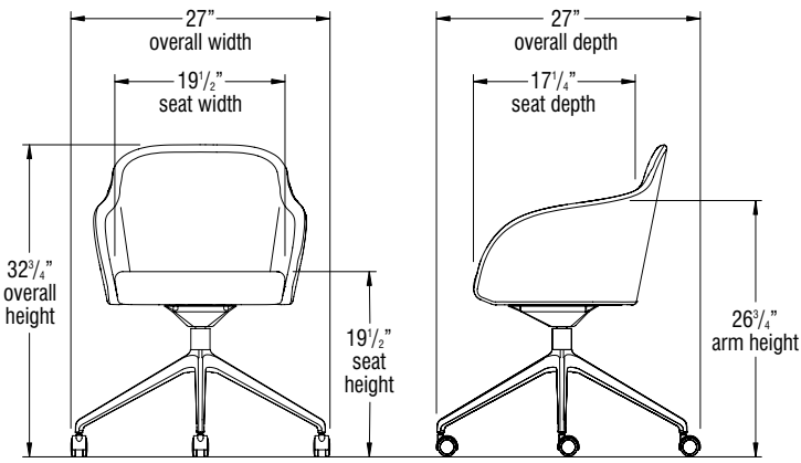
Calida Swivel Chair with Casters
