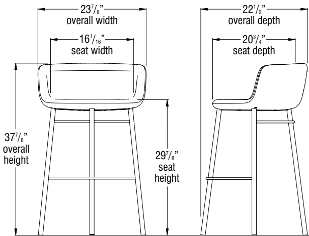
30" Calida 4-Leg Stool
