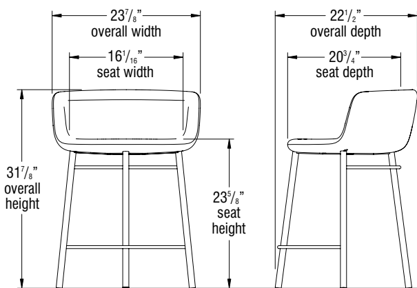
24" Calida 4-Leg Stool
