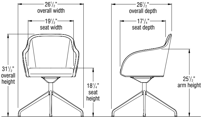
Calida Swivel Chair with Glides
