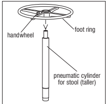
Detail A - Stool Foot Ring
