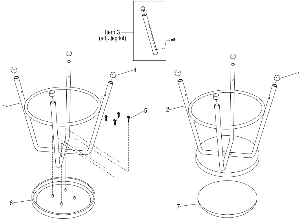
600 Series Stool
