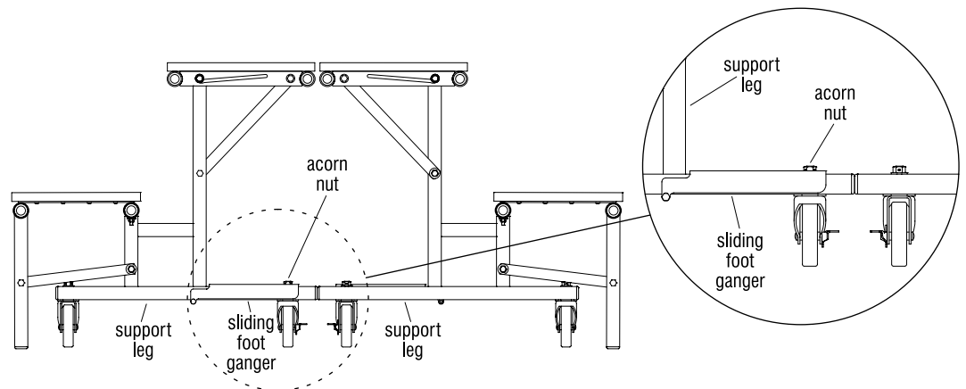
Figure 5 - Ganger Stored Position
