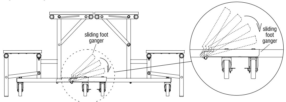
Figure 6 - Ganger Engaged Position
