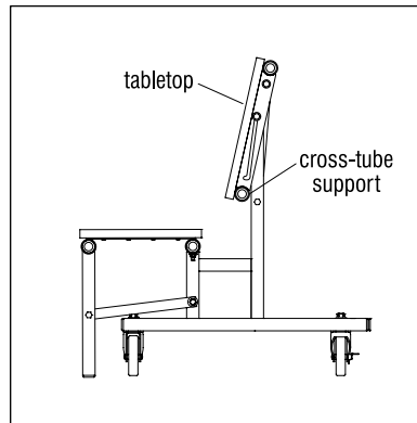
Detail B - Bench Position
