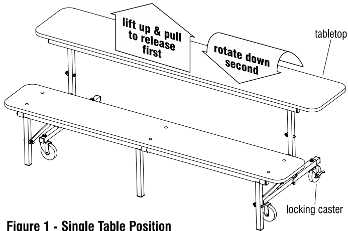
Figure 1 - Single Table Position
