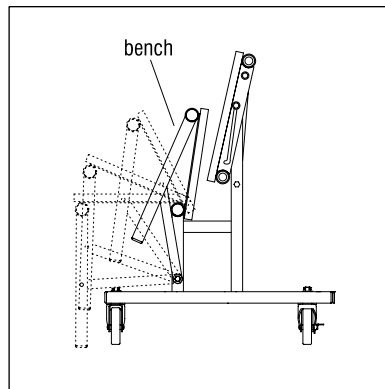
Detail C - Bench-to-Storage Position
