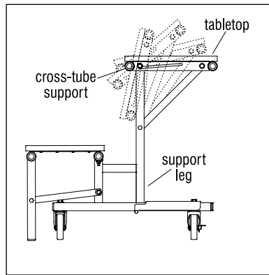
Detail A - Table-to-Bench Position
