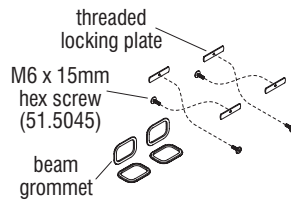
Beam Splice Kit (51.5024)
