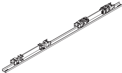
6-2-2 Wire Harness Assembly (51.5040.SIZE.XX)
